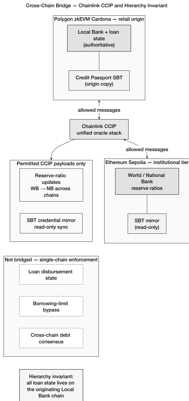
Figure 3.18: Chainlink CCIP cross-chain hierarchy invariant
